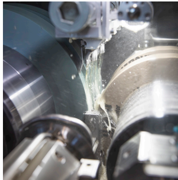
Centerless grinding
