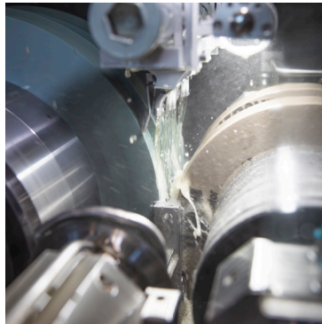
Centerless grinding (picture shows Tschudin proLine 400)
