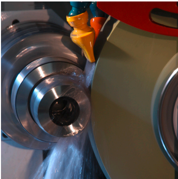
Cylindrical grinding (picture shows Studer machine)
